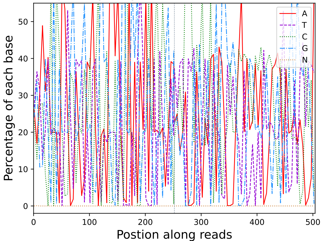
Base percentage along reads (R10711)
